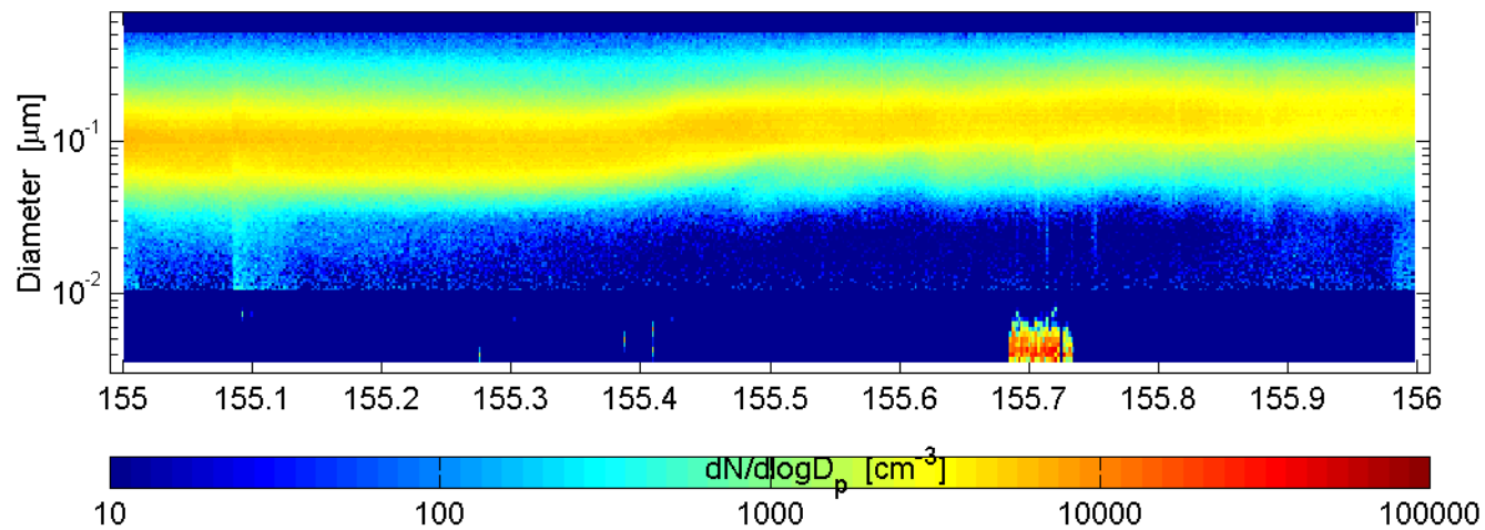
SMPS and nano-SMPS Mace Head (ref: SMPS) : 60604
