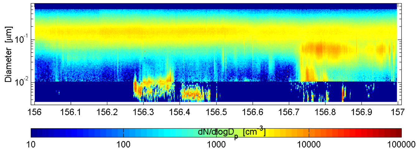
SMPS and nano-SMPS Mace Head (ref: SMPS) : 60605
