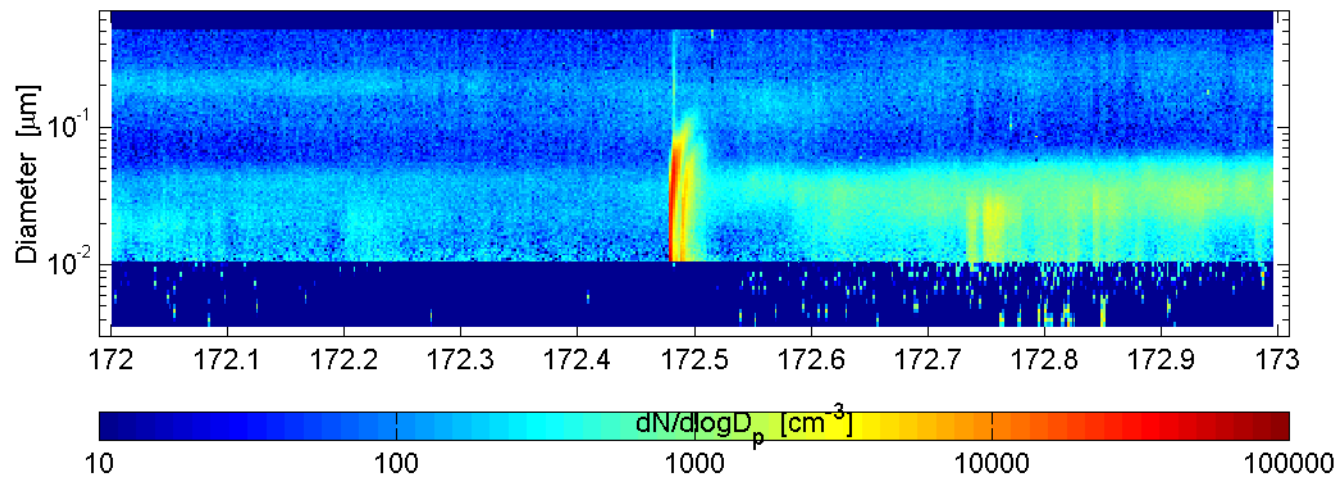
SMPS and nano-SMPS Mace Head (ref: SMPS) : 60621
