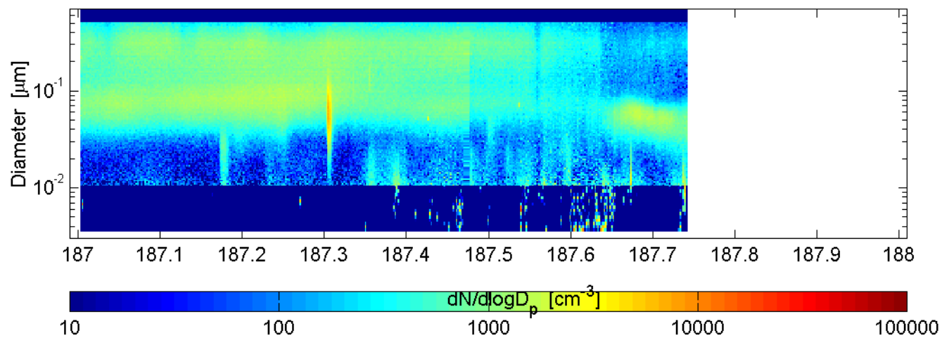
SMPS and nano-SMPS Mace Head (ref: SMPS) : 60706
