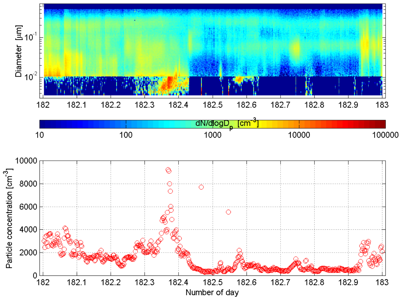
SMPS and nano-SMPS Mace Head (ref: SMPS) : 60701
