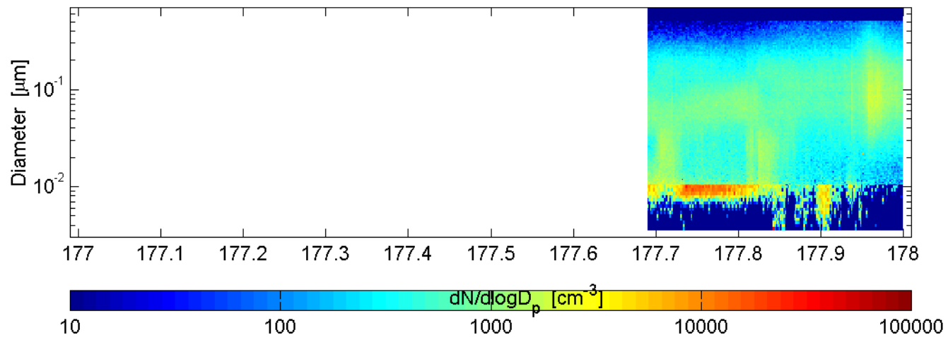
SMPS and nano-SMPS Mace Head (ref: SMPS) : 60626
