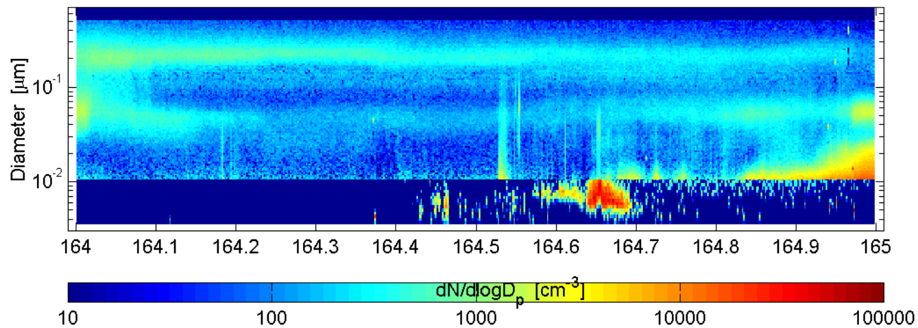
SMPS and nano-SMPS Mace Head (ref: SMPS) : 60613
