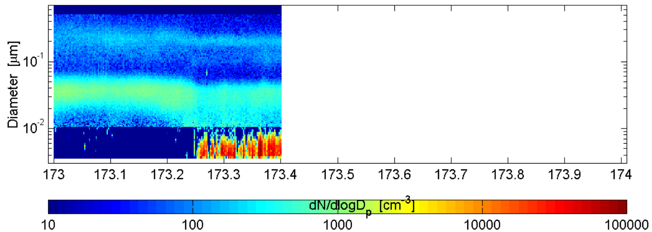
SMPS and nano-SMPS Mace Head (ref: SMPS) : 60622
