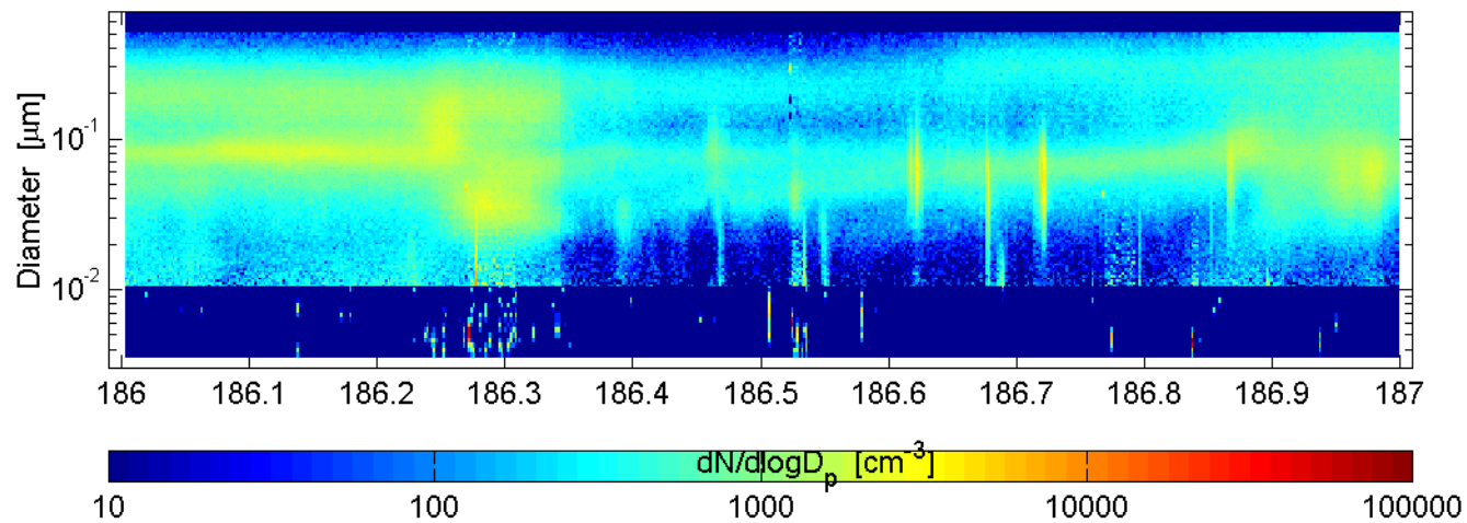
SMPS and nano-SMPS Mace Head (ref: SMPS) : 60705
