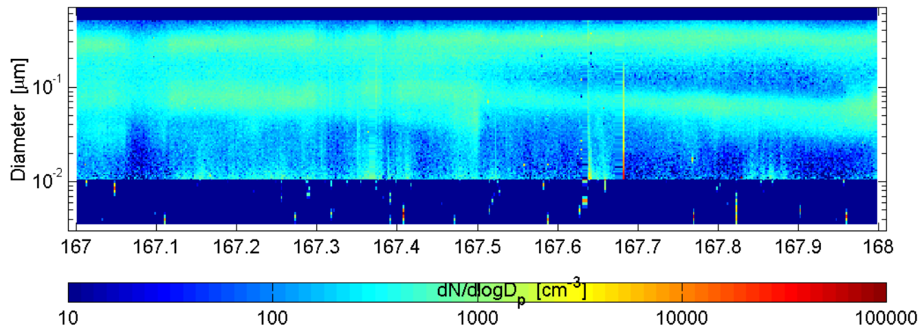
SMPS and nano-SMPS Mace Head (ref: SMPS) : 60616
