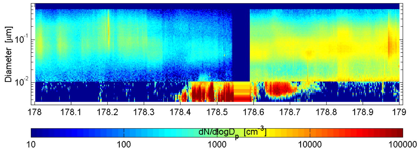
SMPS and nano-SMPS Mace Head (ref: SMPS) : 60627
