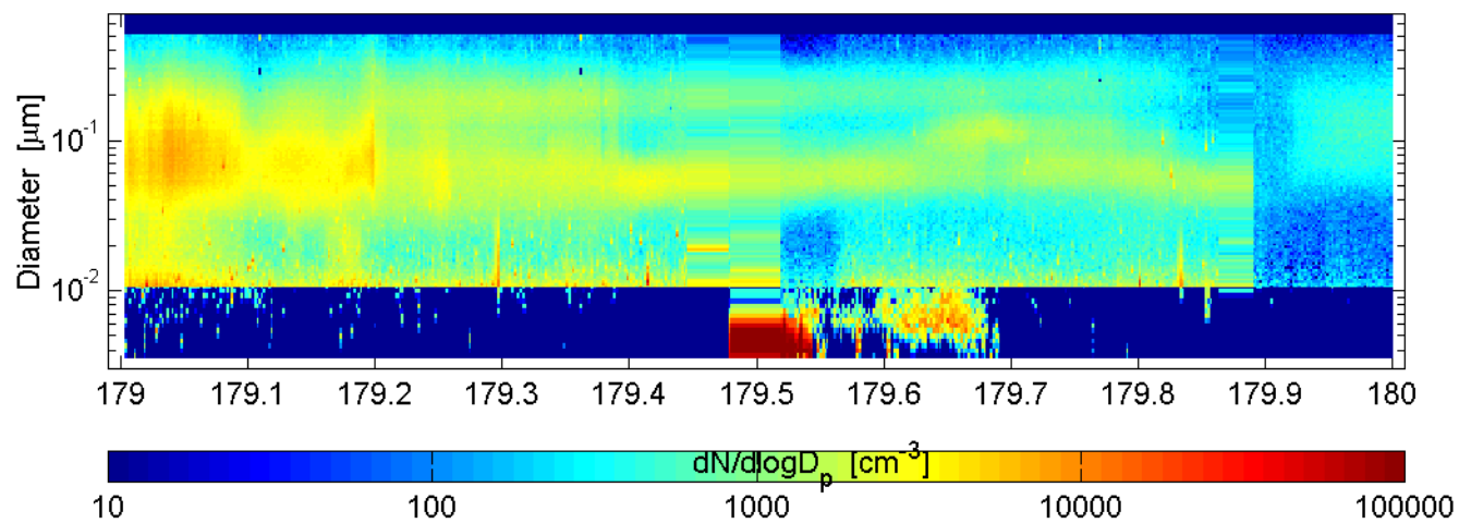
SMPS and nano-SMPS Mace Head (ref: SMPS) : 60628
