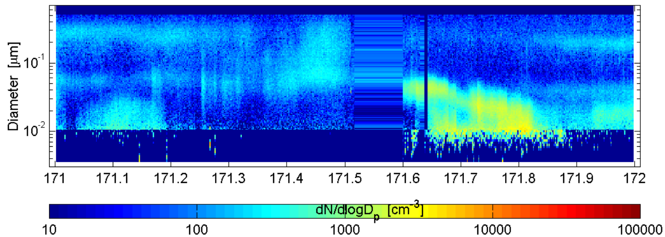
SMPS and nano-SMPS Mace Head (ref: SMPS) : 60620
