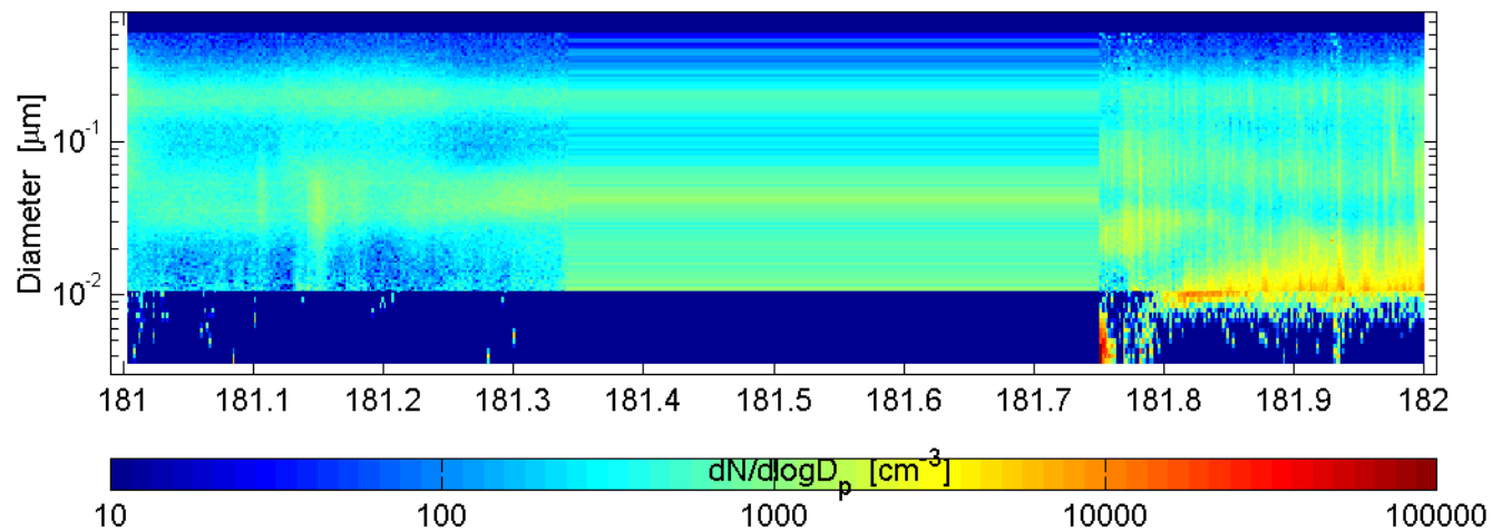
SMPS and nano-SMPS Mace Head (ref: SMPS) : 60630
