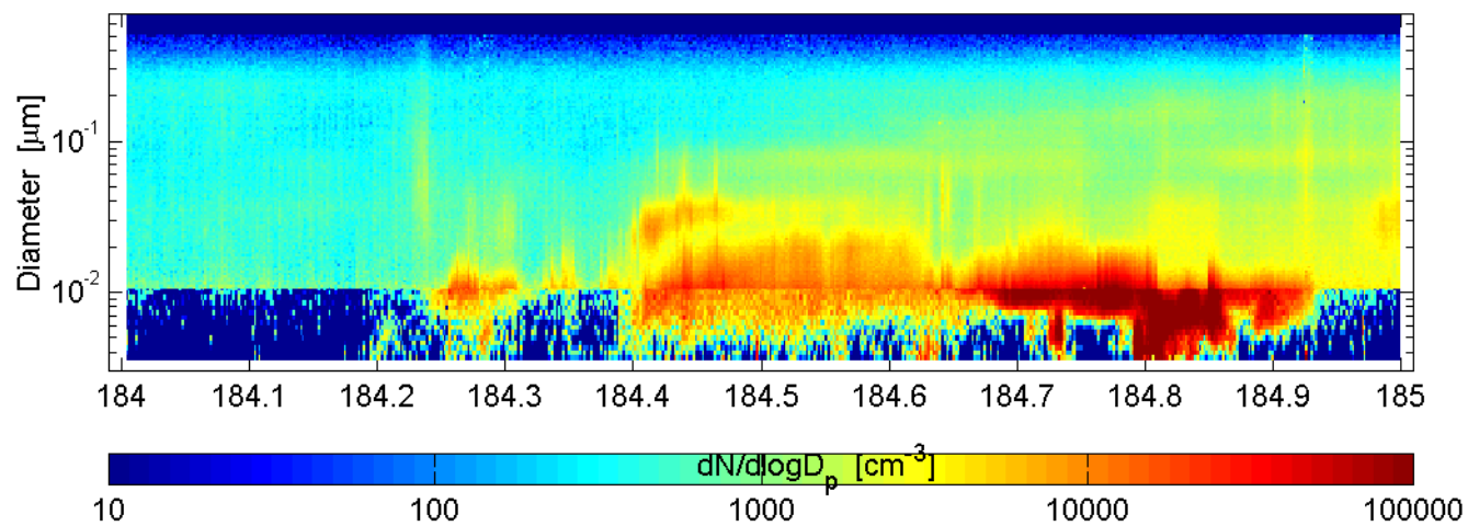
SMPS and nano-SMPS Mace Head (ref: SMPS) : 60703
