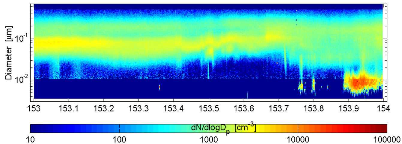
SMPS and nano-SMPS Mace Head (ref: SMPS) : 60602
