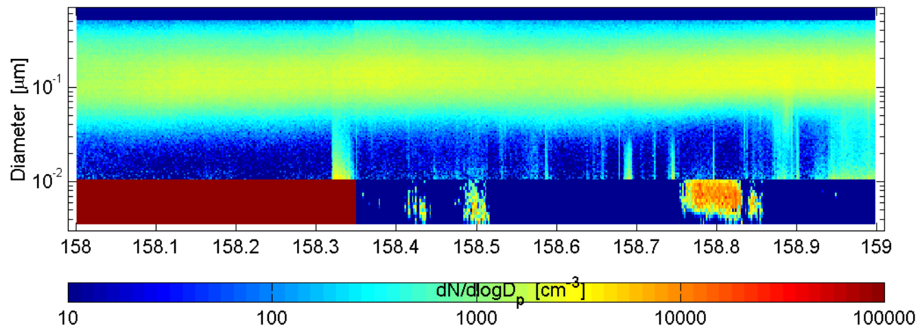
SMPS and nano-SMPS Mace Head (ref: SMPS) : 60607
