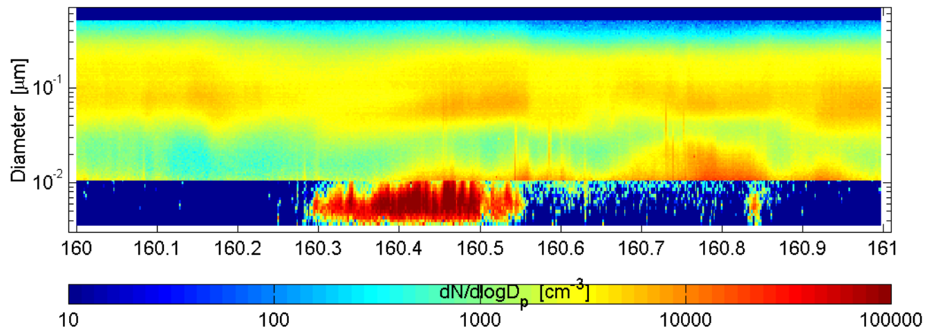
SMPS and nano-SMPS Mace Head (ref: SMPS) : 60609
