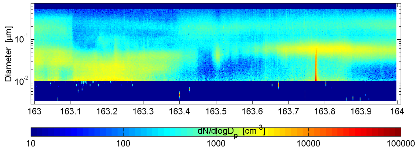
SMPS and nano-SMPS Mace Head (ref: SMPS) : 60612
