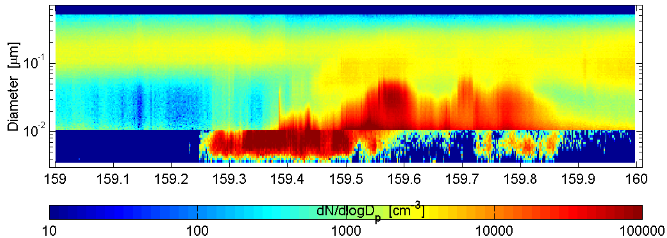
SMPS and nano-SMPS Mace Head (ref: SMPS) : 60608
