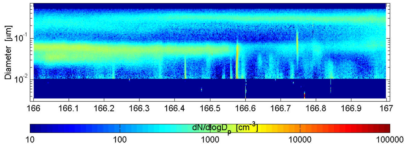
SMPS and nano-SMPS Mace Head (ref: SMPS) : 60615
