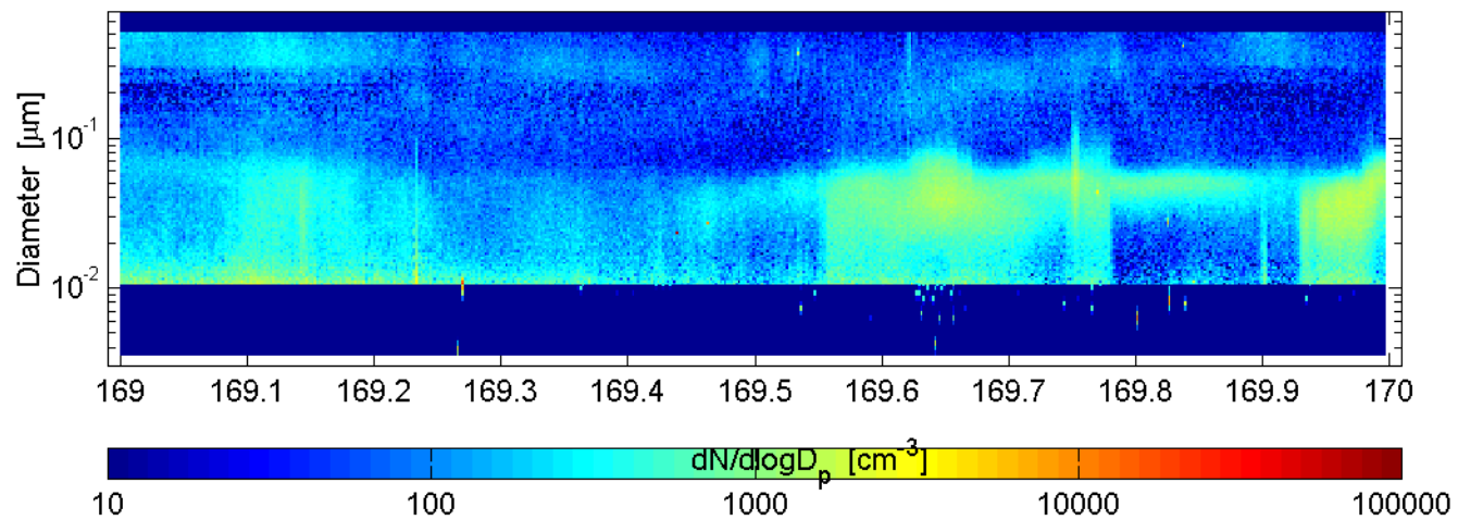
SMPS and nano-SMPS Mace Head (ref: SMPS) : 60618
