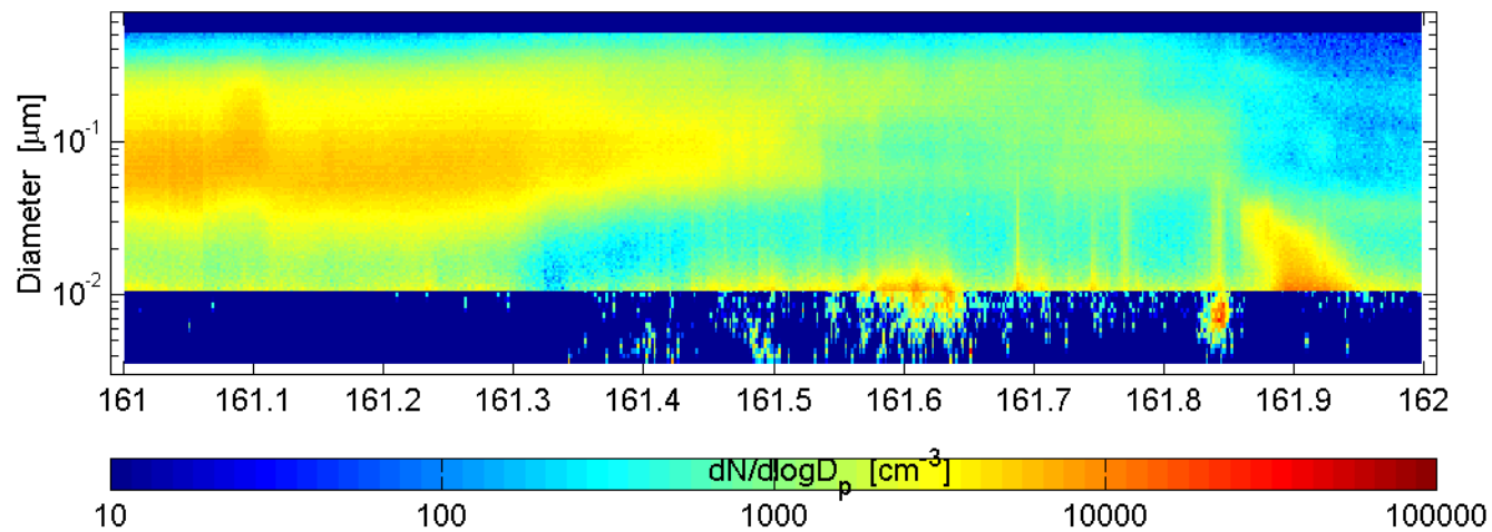
SMPS and nano-SMPS Mace Head (ref: SMPS) : 60610
