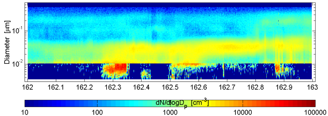
SMPS and nano-SMPS Mace Head (ref: SMPS) : 60611
