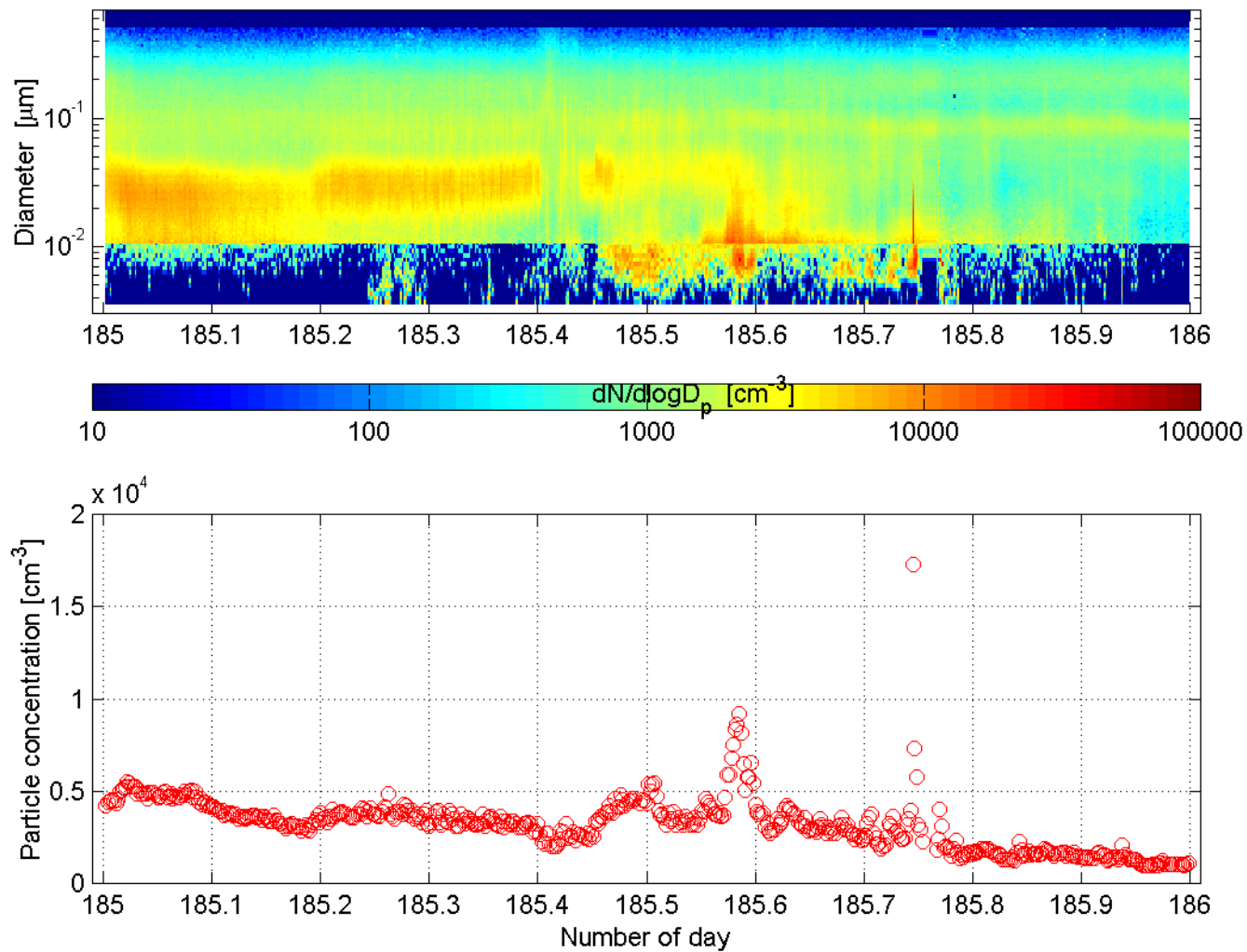
SMPS and nano-SMPS Mace Head (ref: SMPS) : 60704
