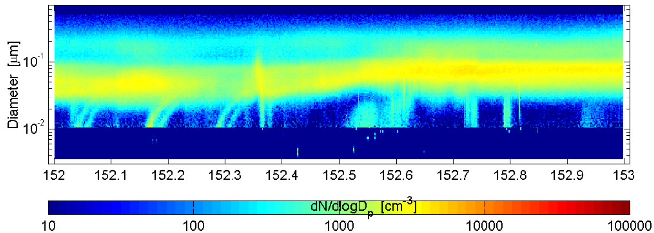
SMPS and nano-SMPS Mace Head (ref: SMPS) : 60601
