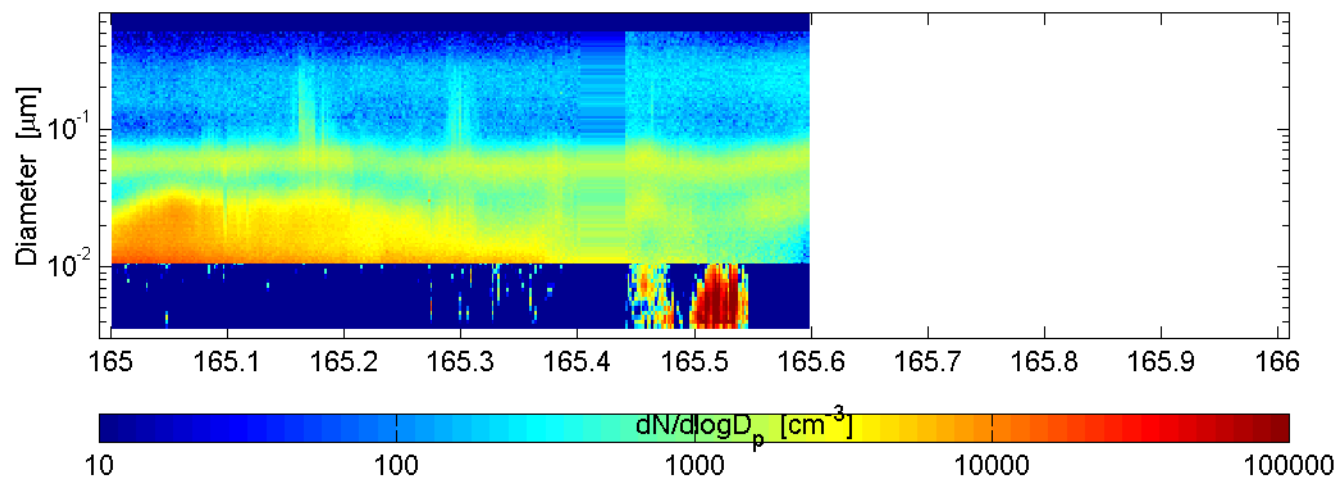
SMPS and nano-SMPS Mace Head (ref: SMPS) : 60614
