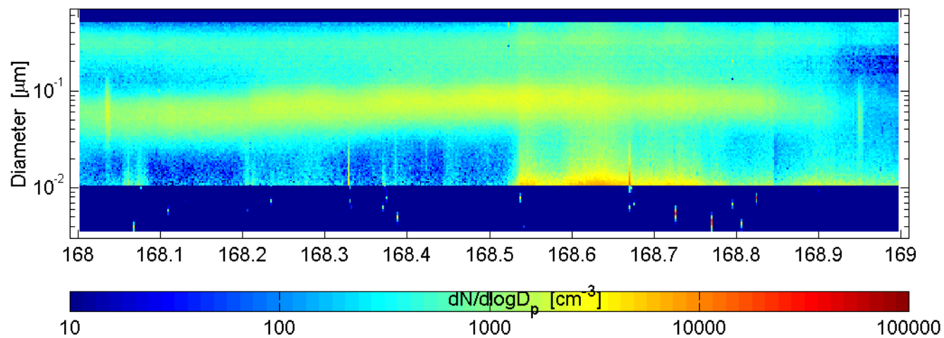
SMPS and nano-SMPS Mace Head (ref: SMPS) : 60617
