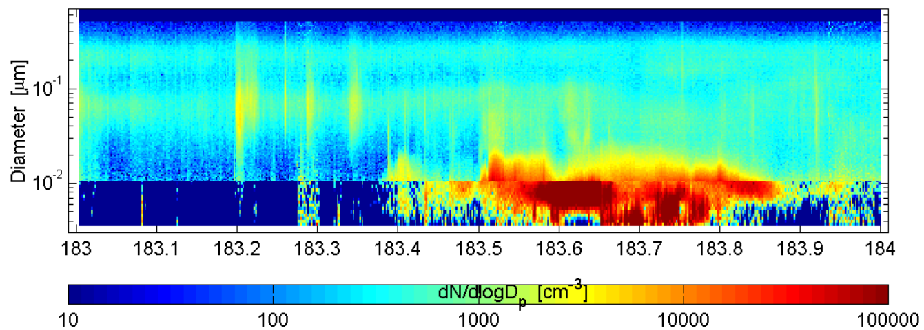
SMPS and nano-SMPS Mace Head (ref: SMPS) : 60702
