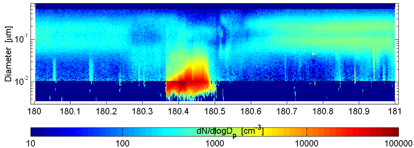
SMPS and nano-SMPS Mace Head (ref: SMPS) : 60629
