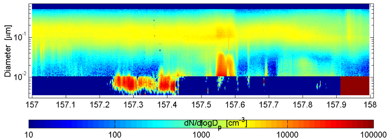
SMPS and nano-SMPS Mace Head (ref: SMPS) : 60606
